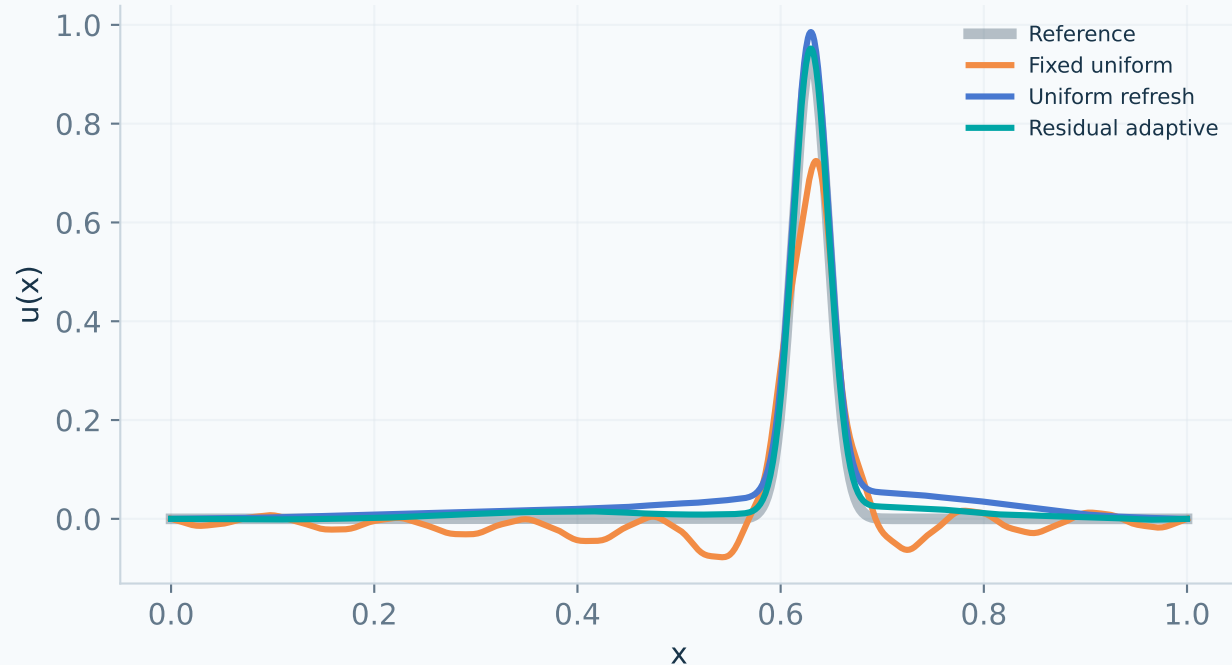
Point placement changes convergence
