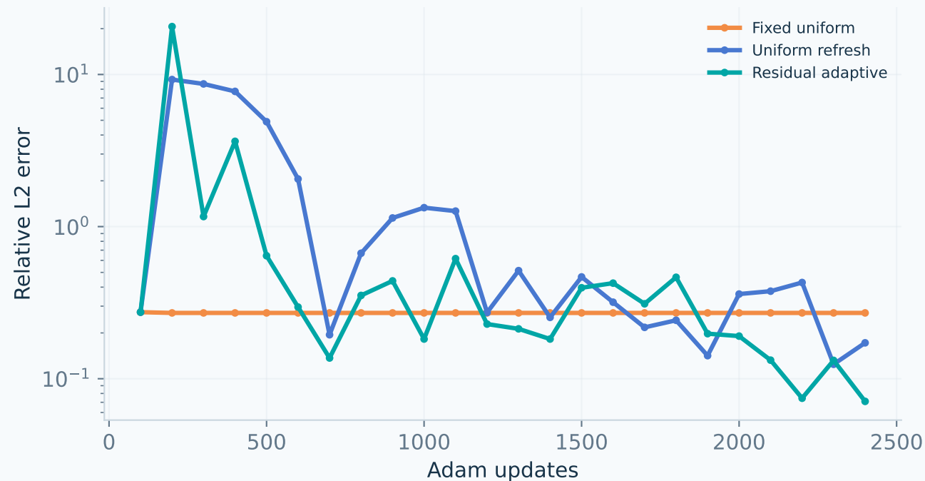
Point placement changes convergence
