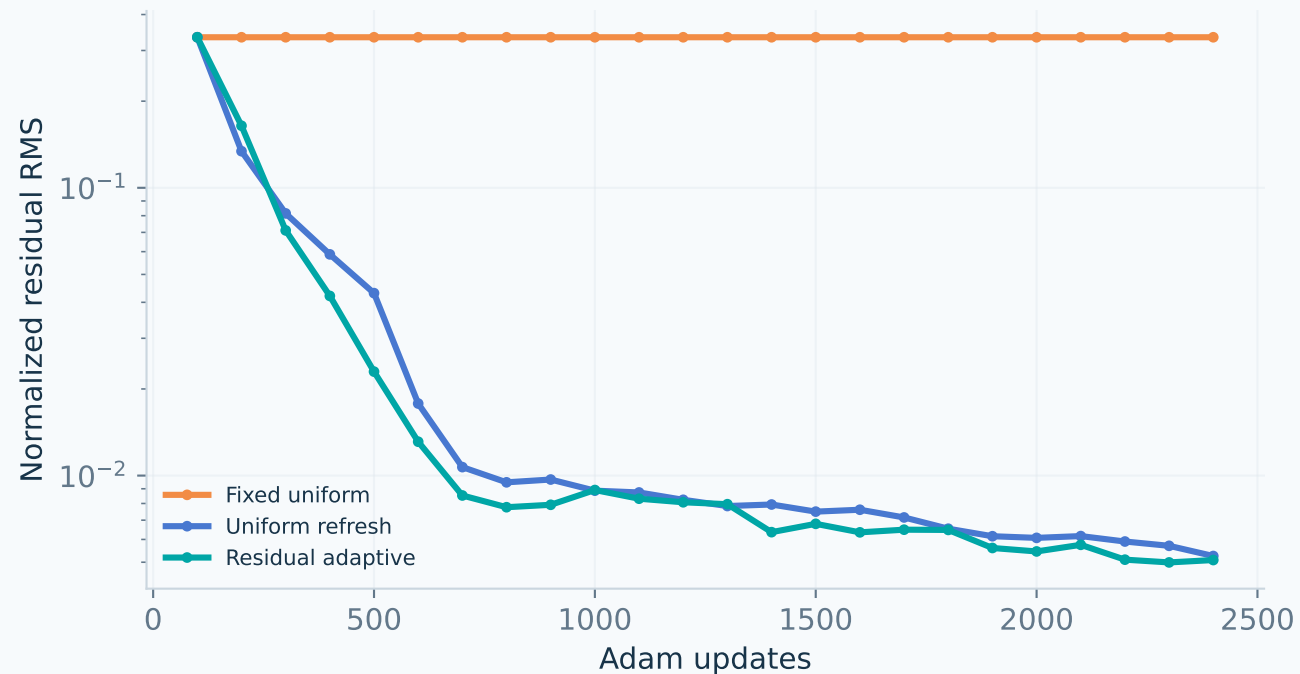
Check between the training points
