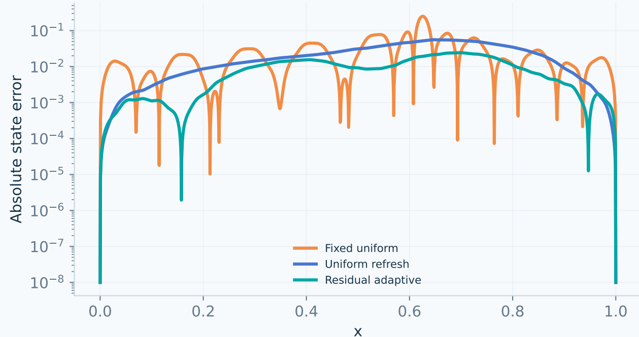
Check between the training points
